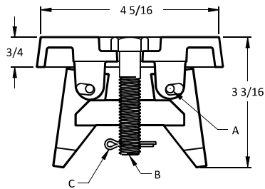
OUTER/OLD STYLE REPAIR LID
