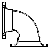
BENDS : MJ X MJ 90° (1/4)
