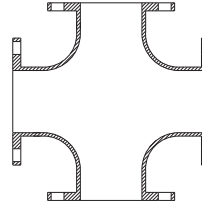
FLANGE CROSS
