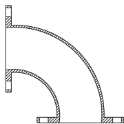
90° LONG RADIUS BENDS
